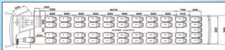
SEATING LAYOUT
